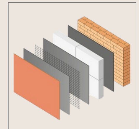
ETICS System
