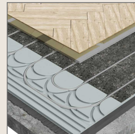
Hydraulic Underfloor Heating
